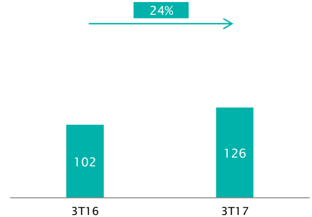
CAPEX
